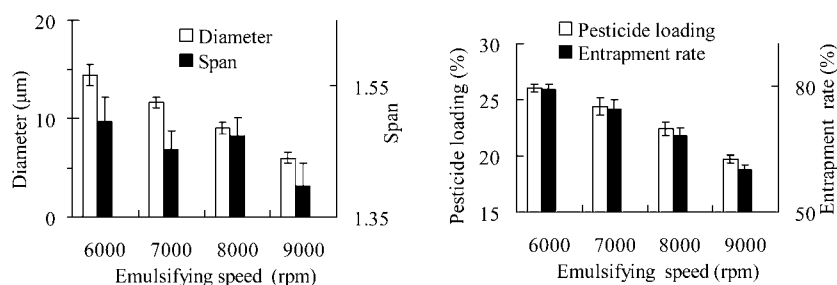
Figure 1. Effects of emulsifying speed on the quality of microcapsules.
