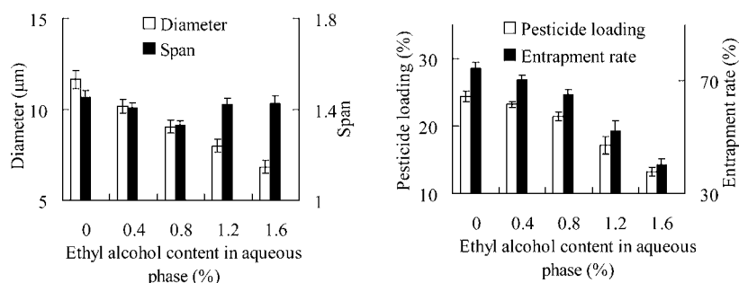
Figure 5. Effects of ethyl alcohol content in external aqueous phase on the quality of microcapsules.
