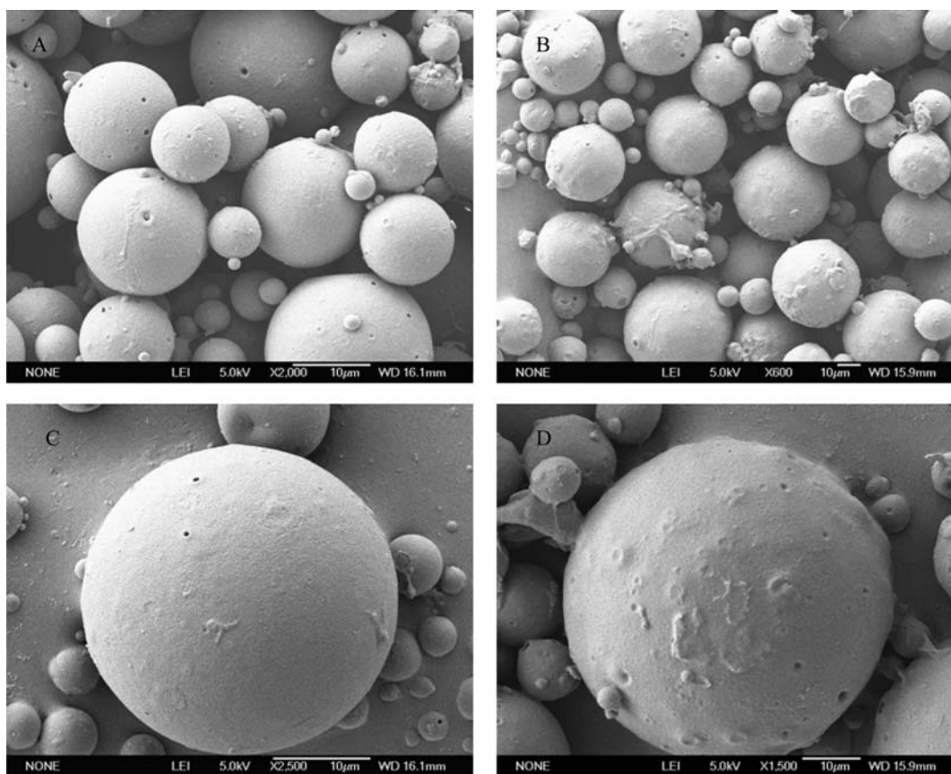
Figure 3. Scanning electron micrographs of microspheres prepared using different internal organic phases: (A, C) internal organic phase was the mixture of dichloromethane with acetone (1:1); (B, D) internal organic phase was dichloromethane alone.
