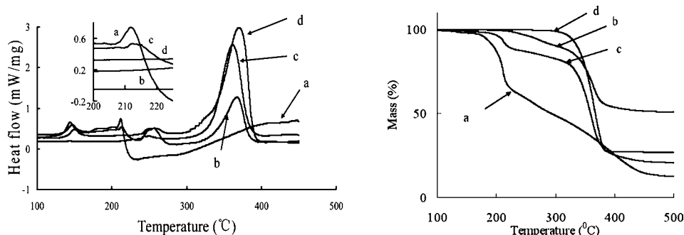
Figure 6. DSC spectrogram diagram (left) and thermal weight loss (right): a, emamectin benzoate; b, PLA microspheres of emamectin benzoate; c, physical mixture of emamectin benzoate and blank PLA microspheres; d, blank PLA microspheres without emamectin benzoate.
