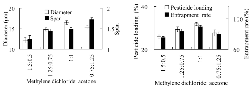
Figure 4. Effects of acetone content in internal organic phase on the quality of microcapsules.
