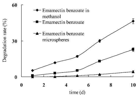
Figure 7. Light degradation curve of emamectin benzoate in PLA microspheres, solid emamectin benzoate, and methanol solution of emamectin benzoate.
